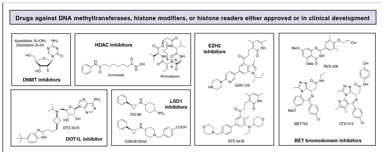
Figure 6. Representative structures of drugs targeting DNA methylation, histone modifications, and histone readers in oncology.
